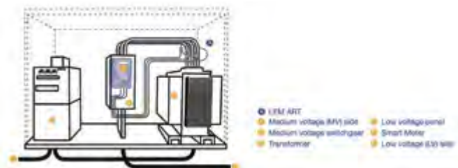
Figure 1: MV/LV Substation
